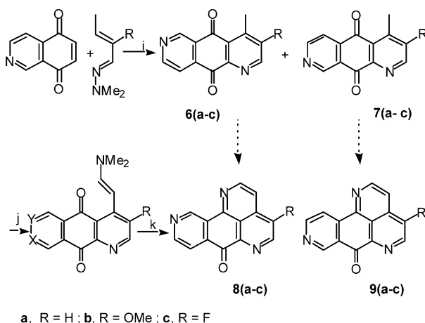
Scheme 2. (i) Toluene, dark, N 2 , rt/MnO 2 , CHCl 3 , rt; (j) DMF-DEA, DMF, N 2 , 120 °C; (k) NH 4 Cl, EtOH, reflux.
