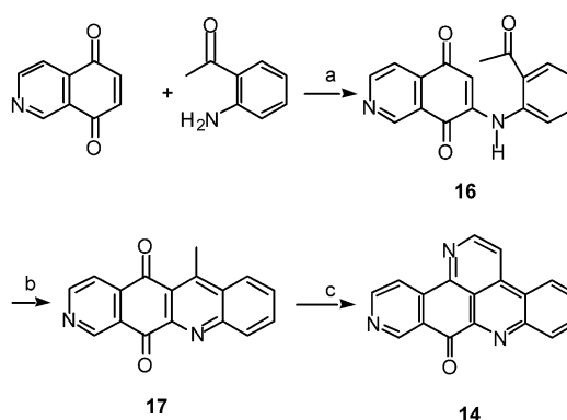
Scheme 4. (a) \text{CeCl}_3 , EtOH, rt, overnight; (b) cc \text{H}_2\text{SO}_4/\text{CH}_3\text{COOH} , reflux, 1 h; (c) DMF-DEA, DMF, \text{N}_2 , 120 °C, 30 min, \text{NH}_4\text{Cl} , MeOH, reflux, 30 min.
