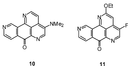
Scheme 3. (a) \text{CHCl}_3 , 1 N NaOH, rt.
