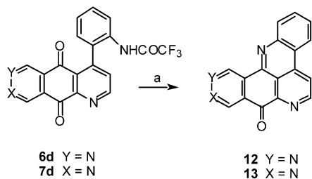
Scheme 3. (a) \text{CHCl}_3 , 1 N NaOH, rt.
